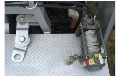
10,000 lbs Line Pull Winch & Pulley
